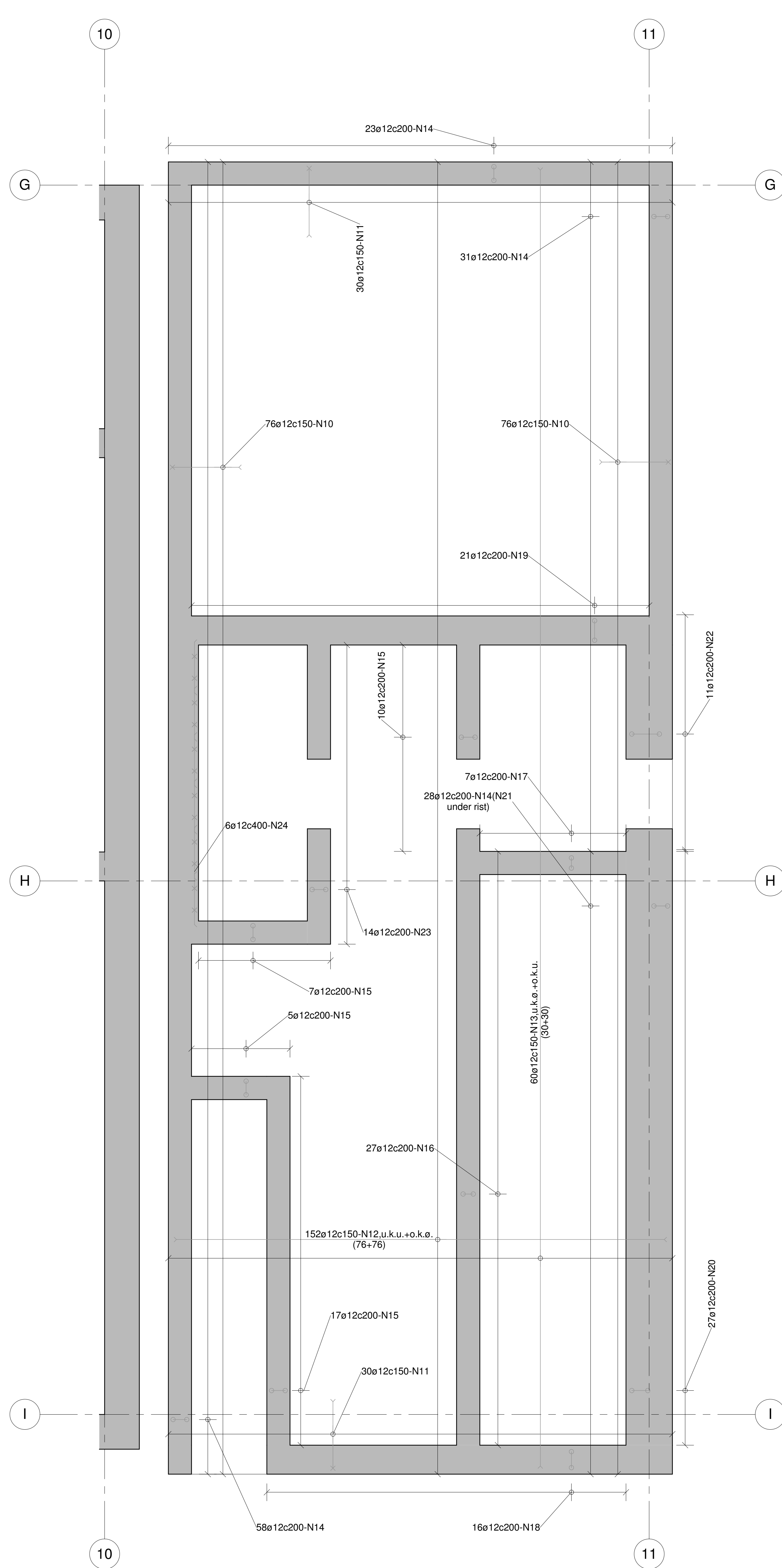
BUNNPLATE 1:20
